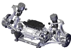
BEDS Integrated E-Chassis
